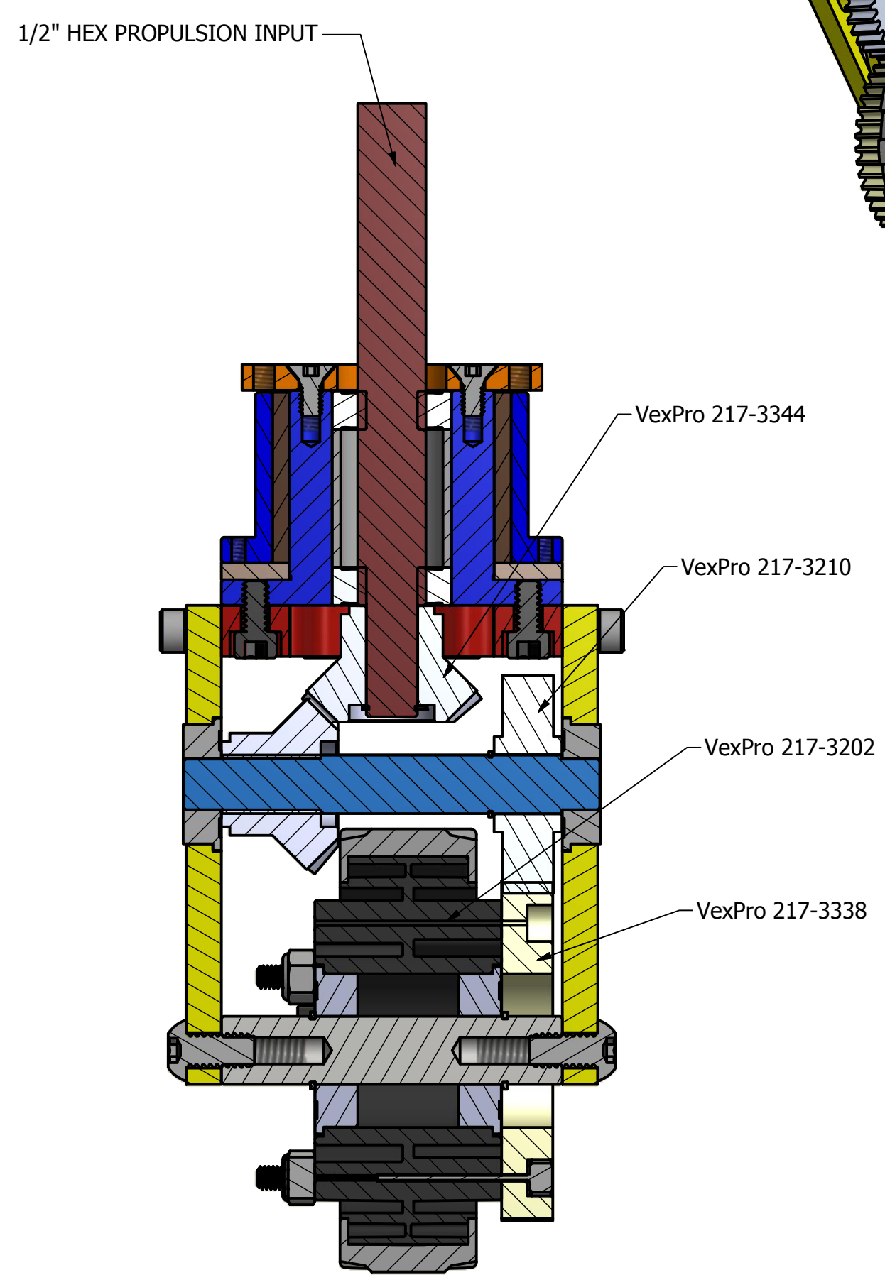
SECTION B-B SCALE 1 : 1
